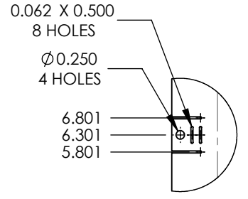
DETAIL C SCALE 1:4
